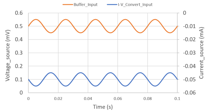
Figure 17. The current and voltage input signals of the BCV circuit.
