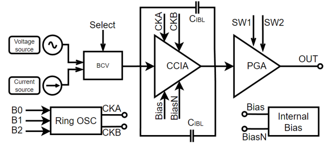
Figure 2. Block diagram of 1-channel AFE.
