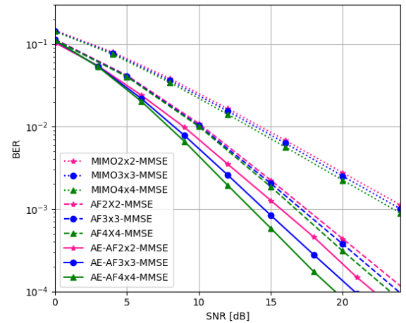
Figure 7. BER comparison between AE-AF-MMSE and the conventional AF-MMSE for N = 2, 3, 4 .
